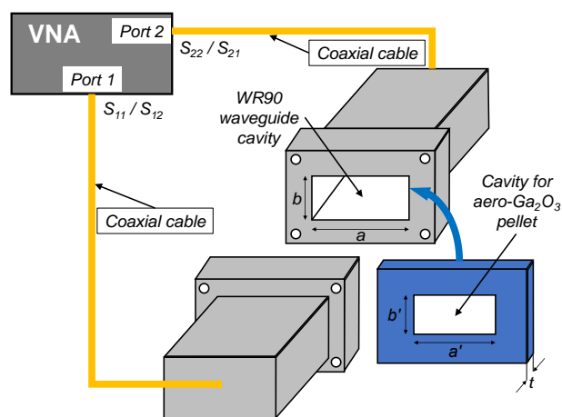
Figure 1. Microwave experimental set-up for X-band characterization of the aero- \text{Ga}_2\text{O}_3 .
