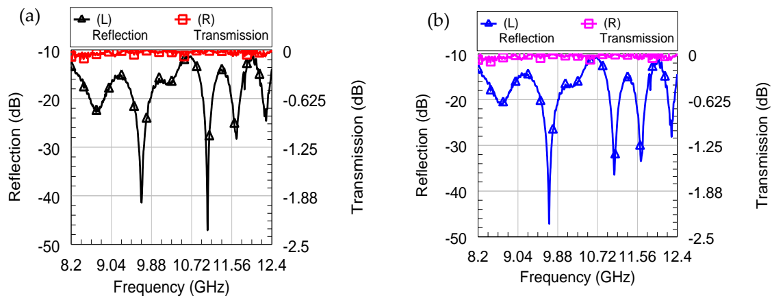
Figure 5. Microwave measurements in X-band for the two cases: (a) without the aero-Ga 2 O 3 pellet and (b) with the aero-Ga 2 O 3 pellet, in terms of reflection (left vertical axis, solid black and blue curves) and transmission (right vertical axis, solid red and pink curves).
