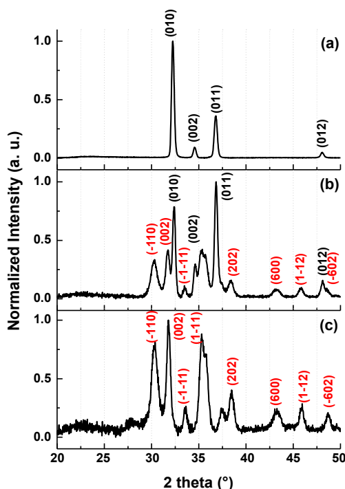
Figure 3. XRD spectra of aero-GaN (a), mixture of GaN and Ga 2 O 3 phases (b) and aero-Ga 2 O 3 (c).
