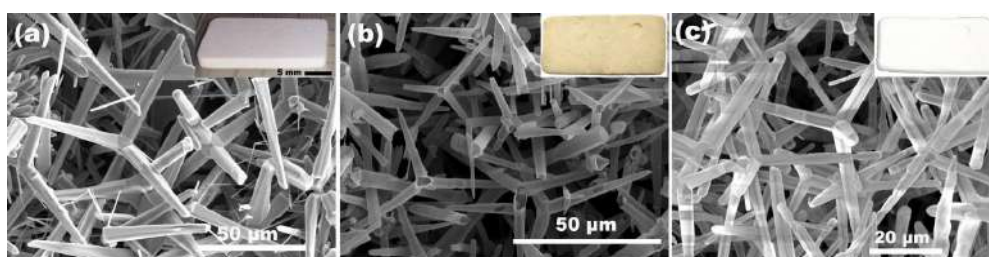
Figure 2. SEM images of (a) initial ZnO template, (b) intermediate aero-GaN, and (c) resulted aero-Ga 2 O 3 nanomaterial. The inset pictures represent the photographs of the pellet samples of ZnO, GaN, and Ga 2 O 3 respectively.
