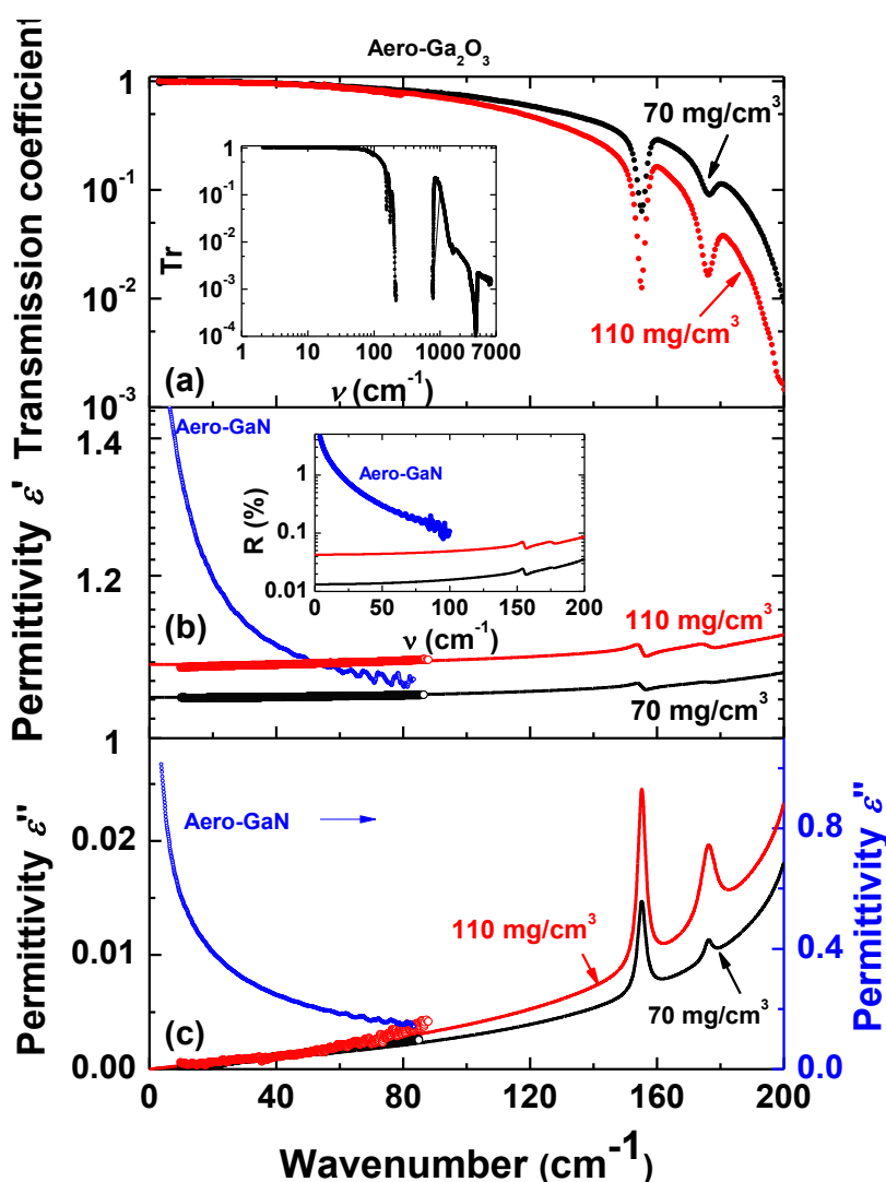
Figure 6. Terahertz spectral characteristics of aero-Ga 2 O 3 samples with two different densities of 70 mg/cm 3 and 110 mg/cm 3 , and aero-GaN sample with the density of 15 mg/cm 3 (data from [22]): transmission coefficient Tr (a), real \epsilon' (b) and imaginary \epsilon'' (c) parts of dielectric permittivity. Open dots on panels (b) and (c) present THz data for permittivity. Inset in panel (a): spectrum of transmission coefficient measured at frequencies up to 7000 cm -1 . Inset in panel (b): spectra of reflection coefficient calculated basing on measured spectra of real and imaginary parts of dielectric permittivity using standard Fresnel expressions [14].
