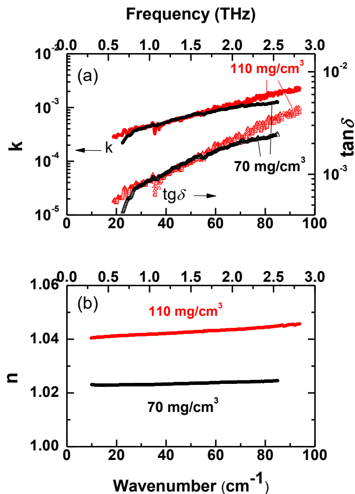
Figure 7. Spectra of terahertz electrodynamic characteristics of aero-Ga 2 O 3 samples with two different densities of 70 mg/cm 3 and 110 mg/cm 3 : imaginary k (a) and real n (b) parts of complex refractive index n + ik and dielectric loss tangent \tan\delta (panel a, triangles).
